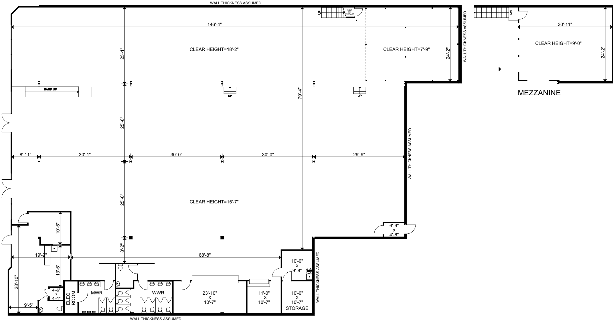
FLOOR 1
